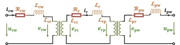
Fig. 2. Equivalent Circuit for a BDFIG
