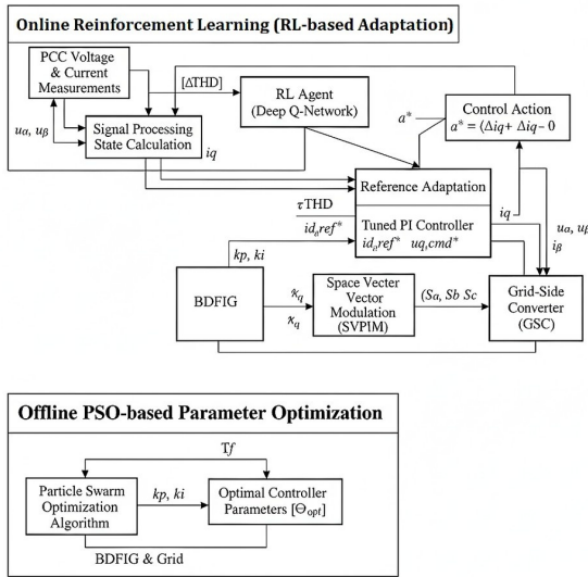
Fig. 3. Proposed PSO Controller with an RL agent
