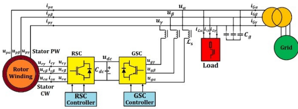
Fig. 1. Block diagram of BDFIG
