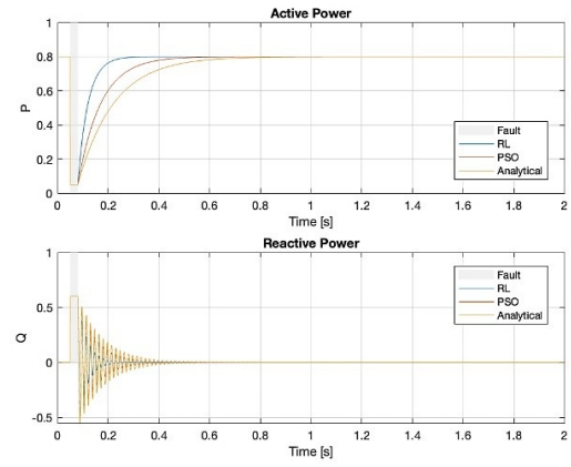
Fig. 7. Active & Reactive Power—Proposed vs Fault, PSO, Analytical.
