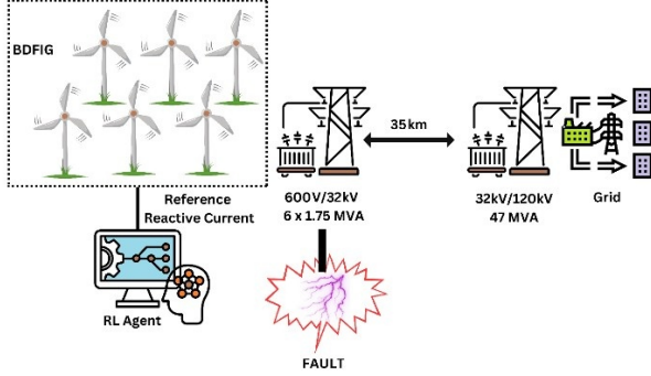
Fig. 5. Block diagram of the simulation model.
